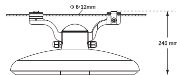
Suspended Mounted
